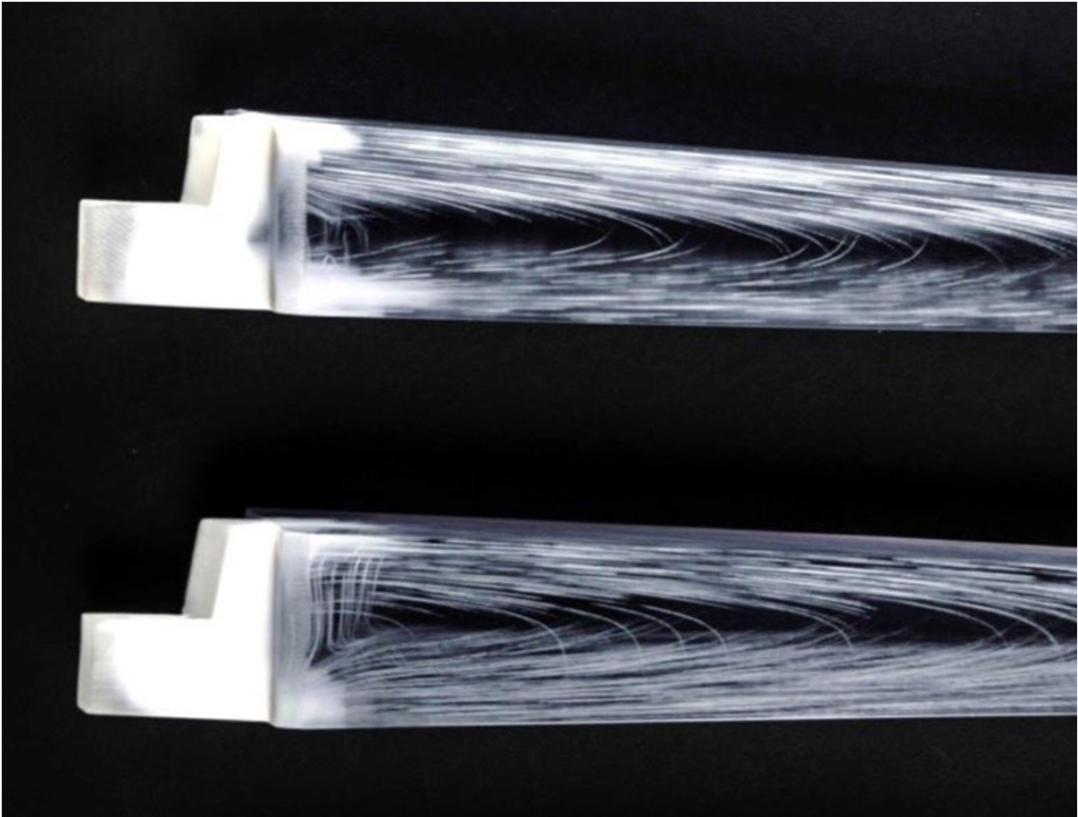
DManD researchers explored the structural behavior of traditional timber joinery systems using a custom design, analysis and slicer tools, and the GrabCAD Voxel Print utility. Photography by Teo Jansen.
