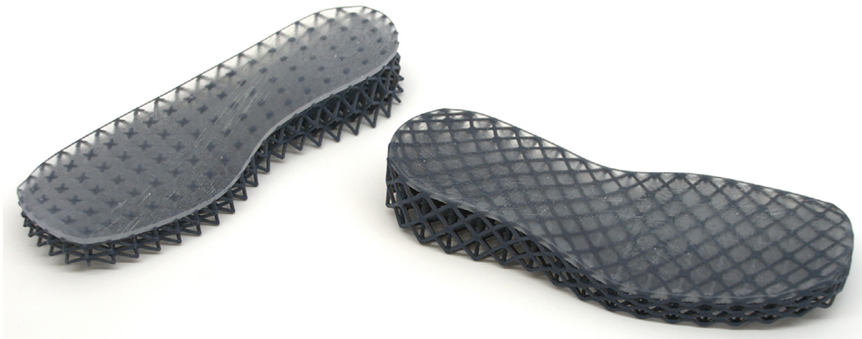
DManD researchers created multi-material soft-lattice structures for this footwear prototype using a custom design, analysis and slicer tools to spatially control stiffness and non-linear
